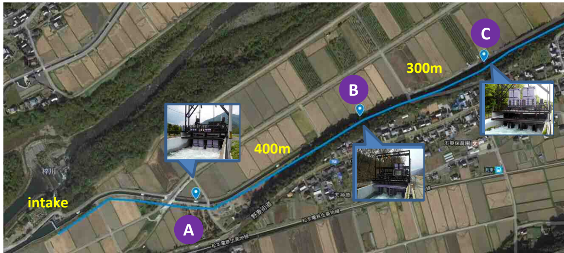
A Irrigation canal, Nagano pref. / rated output : 37kW x 2units / Mar. 2017
